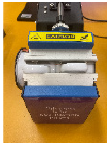
Enamel mug - max. size 200x60 mm, heat press temp. 200 C°, time 275 sec. When pressing enamel mug, use another mug to keep pressure even!
